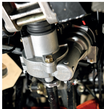
Left: electric motor attaches to a new part in the column. Above: dial allows amount of assistance to be tweaked
